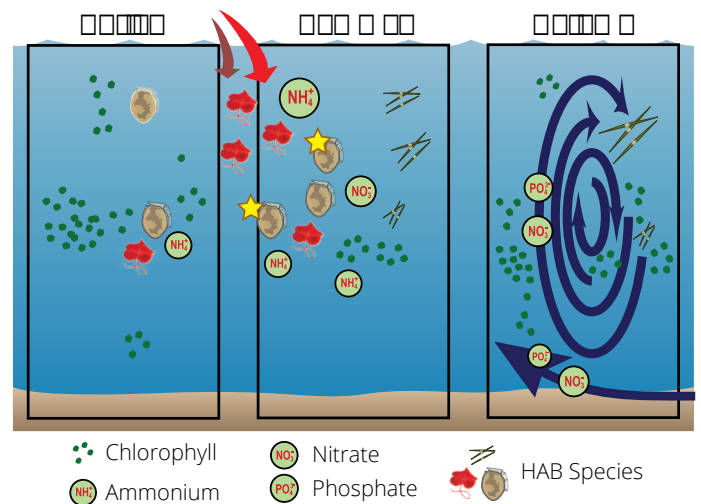
Conceptual diagram outlining the chemical, biological, and physical processes that occur in the study region.
